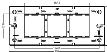
6 Module with Partition
