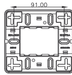
Cutout size– 72mm x 57mm Code No: 373003 3H module – 4.5" X 5"
