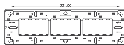
Cutout size– 296mm x 57mm Code No: 373010 12H module – 4.5" X 15"
