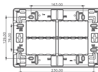
Cutout size– 196mm x 112mm Code No: 373013 16 module – 7.5" X 11"
