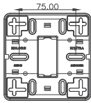
Cutout size– 28mm x 57mm Code No: 373001 1H module – 4.5" X 4.5"
