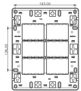
Cutout size– 152mm x 167mm Code No: 373014 18 module – 8.5" X 10.5"
