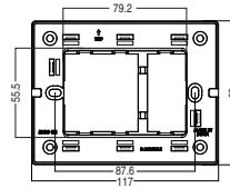
3 Module with Partition
